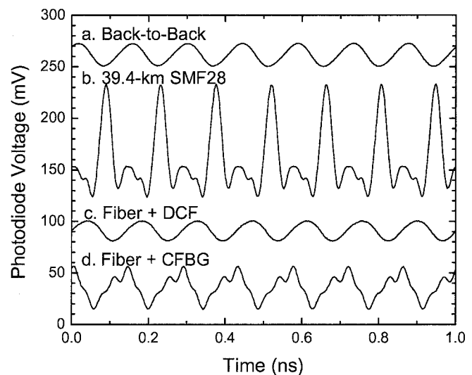
Fig. 6. 1550.000-nm demodulated time-domain waveforms at various points in the angle-modulated link: (a) back-to-back, (b) after 39.4 km of standard fiber, (c) the standard fiber compensated with DCF, and (d) the standard fiber compensated with the CFBG.
